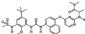
2-(4-{4-[3-(5-tert-Butyl-3-methanesulfonylamino-2-methoxy-phenyl)-ureido]-naphthalen-1-yloxy}-pyrimidin-2-ylamino)-N,N-dimethyl-propionamide;
